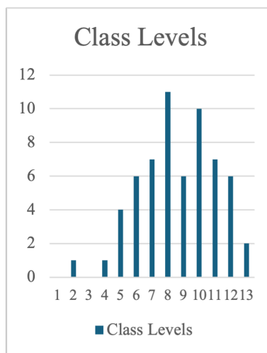
Figure 2. Number of studies (y-axis) investigating different class levels (x-axis)
